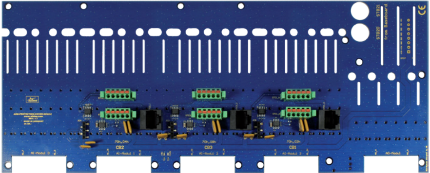
Abb. 5: ADQ-PROTECTION-COVER-SCU 2.0
