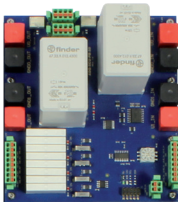
Abb. 3: Powerboard ADQ-SCU-PB-50
