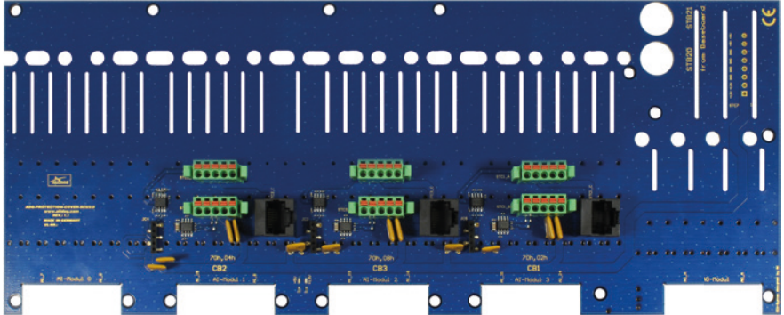
Fig. 5: ADQ-PROTECTION-COVER-SCU 2.0
