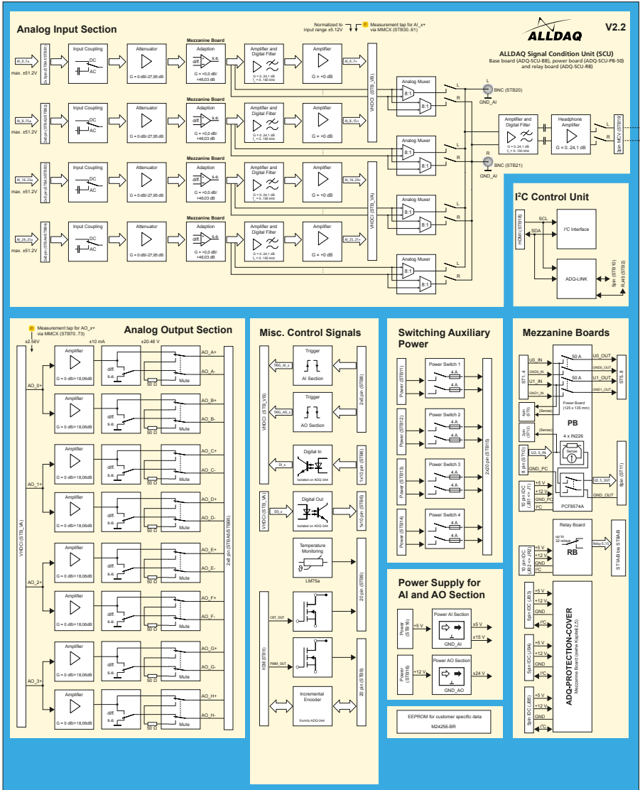
Fig. 1: Block diagram ADQ-SCU
