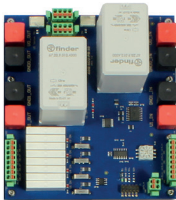
Abb. 3: Powerboard ADQ-SCU-PB-50
